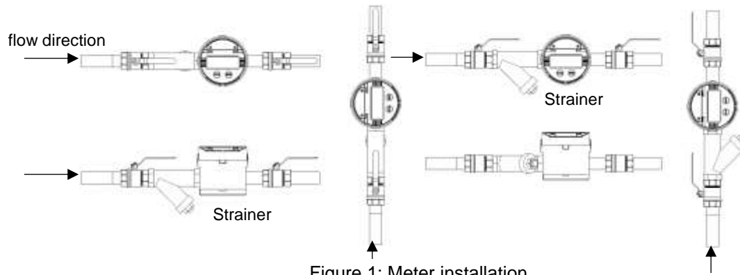
Figure 1: Meter installation
